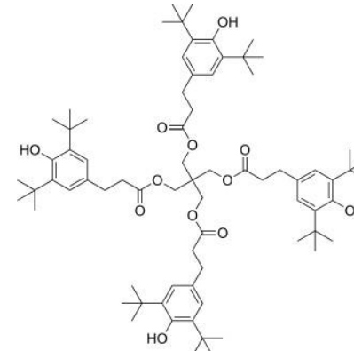
Primary antioxidant
